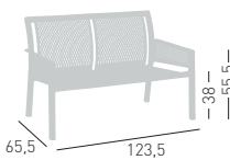
MINUSH SOFA 2 seat technopolymer bench with co-injected metal frame. Panca 2 posti in tecnopolimero con telaio metallico co-iniettato.
