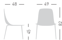
ALHAMBRA NA Technopolimer padded and upholstered shell. Chromed, black or white painted metal frame. Scocca in tecnopolimero, imbottita e rivestita. Telaio in metallo cromato, verniciato nero o bianco.
