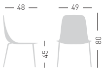
COLORFIVE NA Techno polymer upholstered shell, chromed or painted metal frame. Scocca in tecnopolimero rivestita, telaio in metallo cromato o verniciato.
