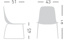
COLORFIVE ST Techno polymer upholstered shell, chromed or painted metal frame. Scocca in tecnopolimero rivestita, telaio in metallo cromato o verniciato.
